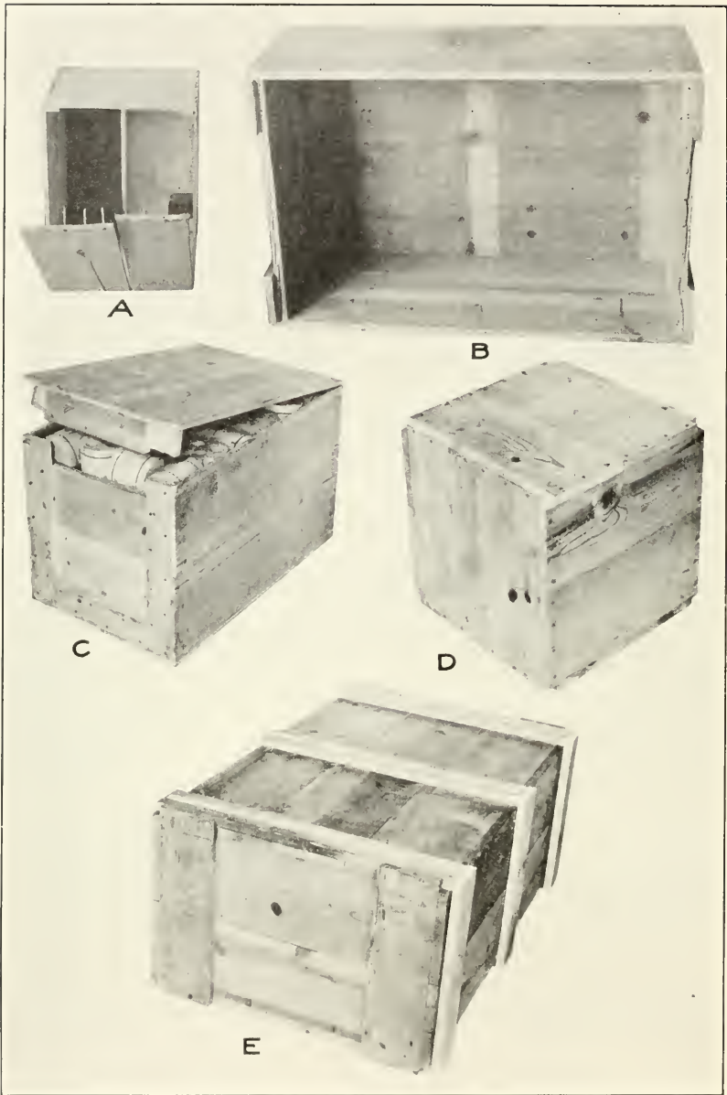
A and B, Typical failure of the ends of styles 1 and 5 nailed boxes by splitting at the nails; C, failure of style 2 box by splitting of end at edge of eleat; D, 3-way corner or so-called hardware type of box; E, box reinforced with wooden battens
